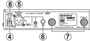
Figure 2 - RE-2 Back Panel
