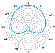
Uni-directional (at 1kHz)
