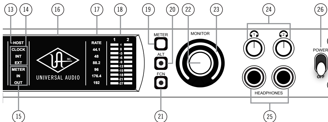
Apollo 8p front panel (right portion)
