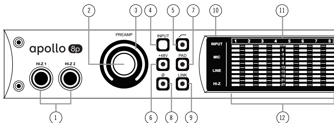
Apollo 8p front panel (left portion)
