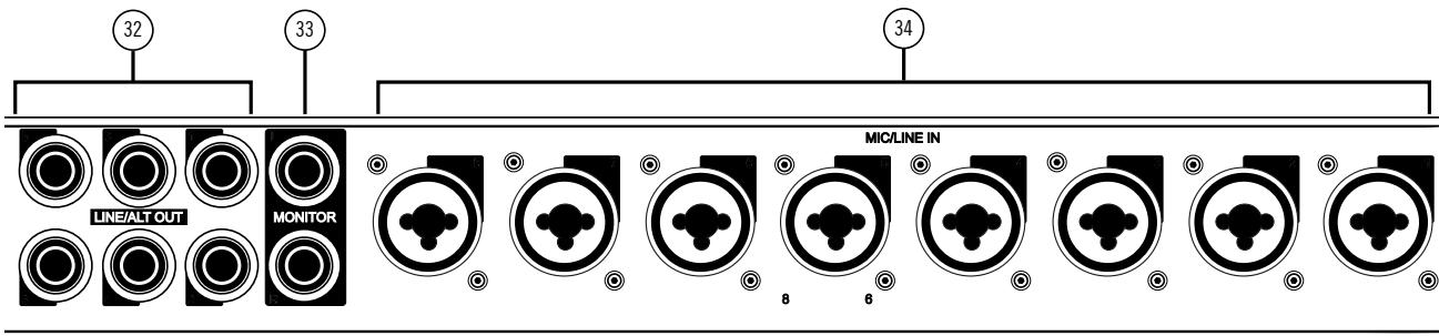
Apollo 8p rear panel (analog portion)
