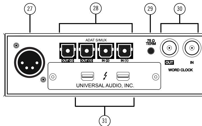
Apollo 8p rear panel (digital portion)
