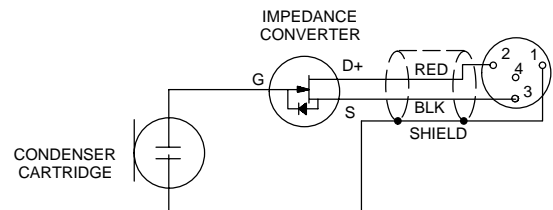
MICROPHONE WIRING DIAGRAM
