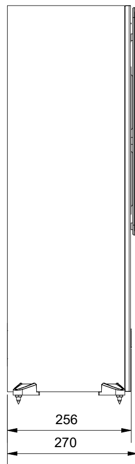
SIDE
