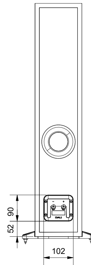
BACK
