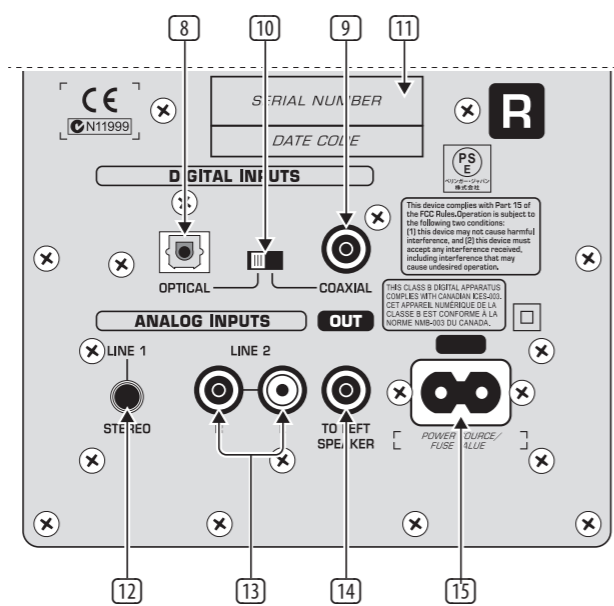
Rear panel (right monitor)
