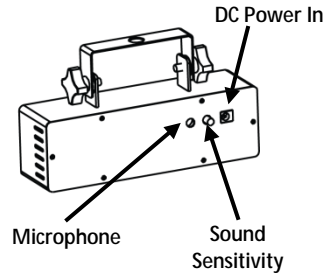
Back Panel View
