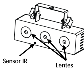
Vista frontal
