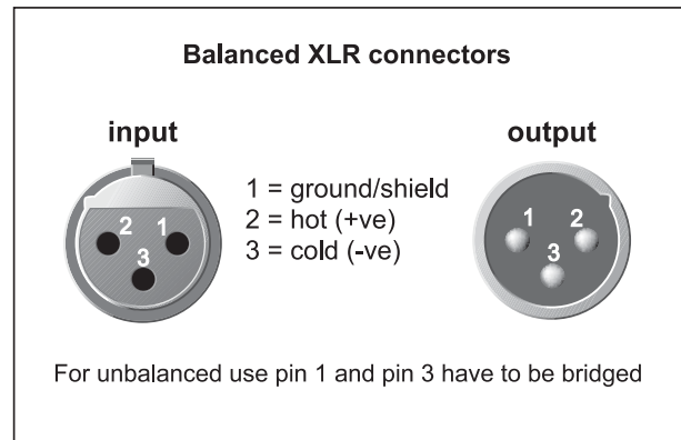
Fig. 5.1: XLR connectors
