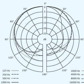
Polar diagram MMD 835-1
