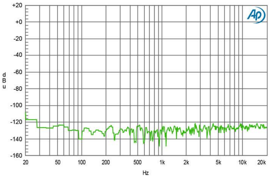
Radial PZ-DI Noise Spectrum
