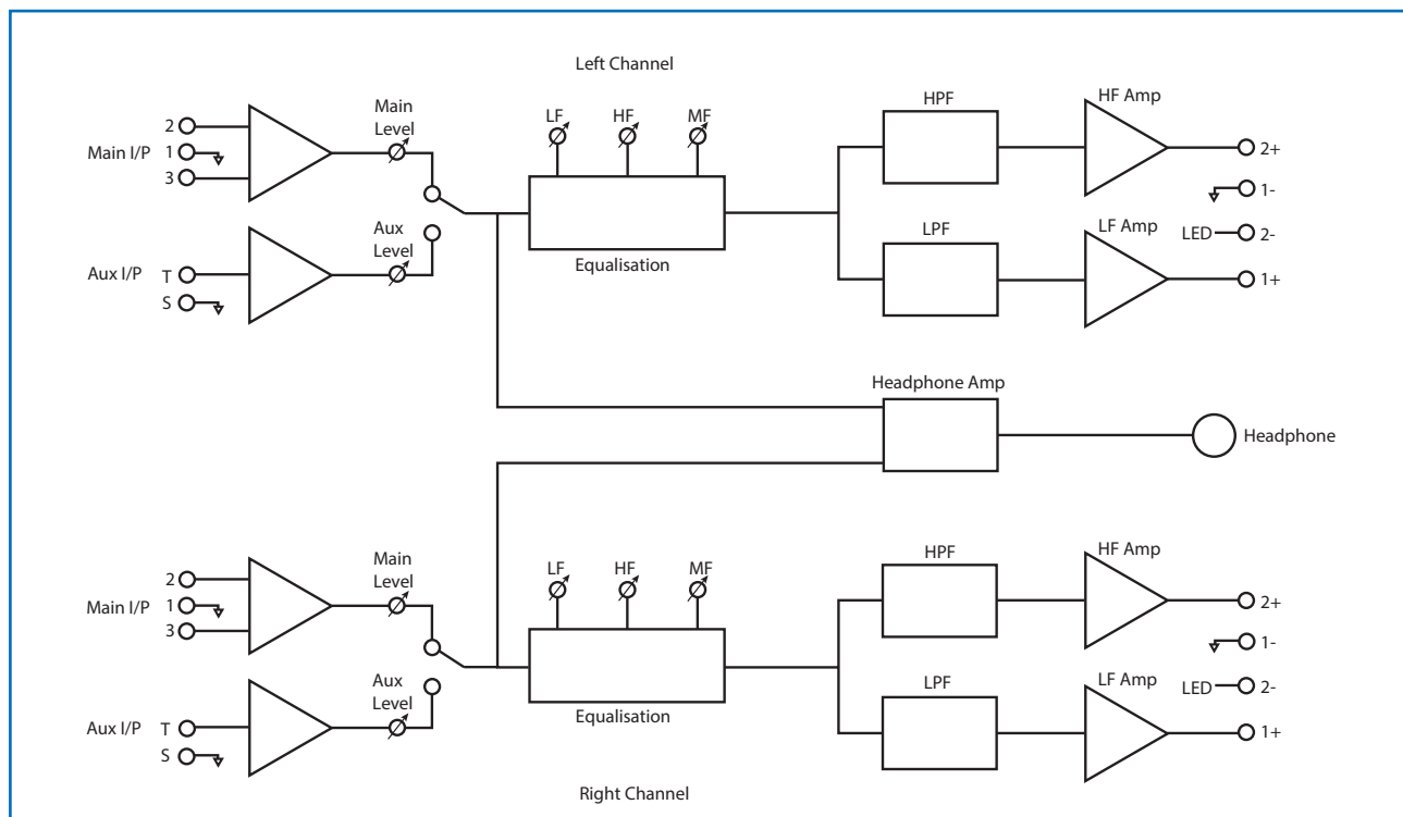
Egg 150 Monitoring System schematic
