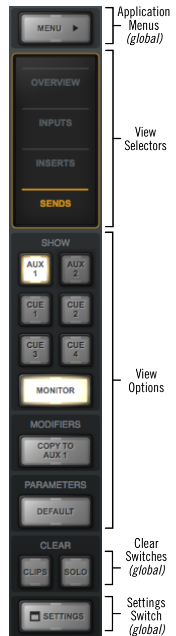
The View Column as it appears in SENDS View
