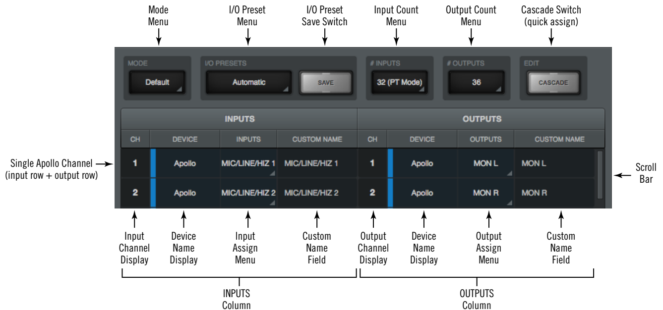
The main Core Audio panel elements
