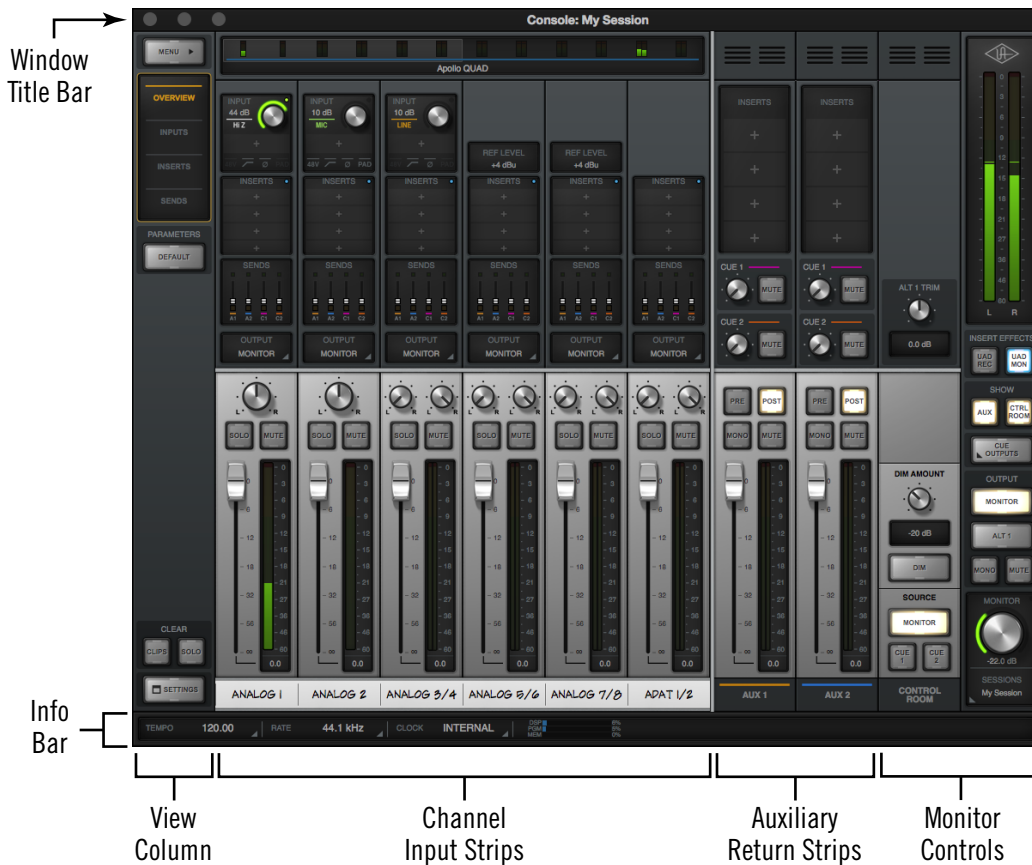
Console’s main window and controls layout
