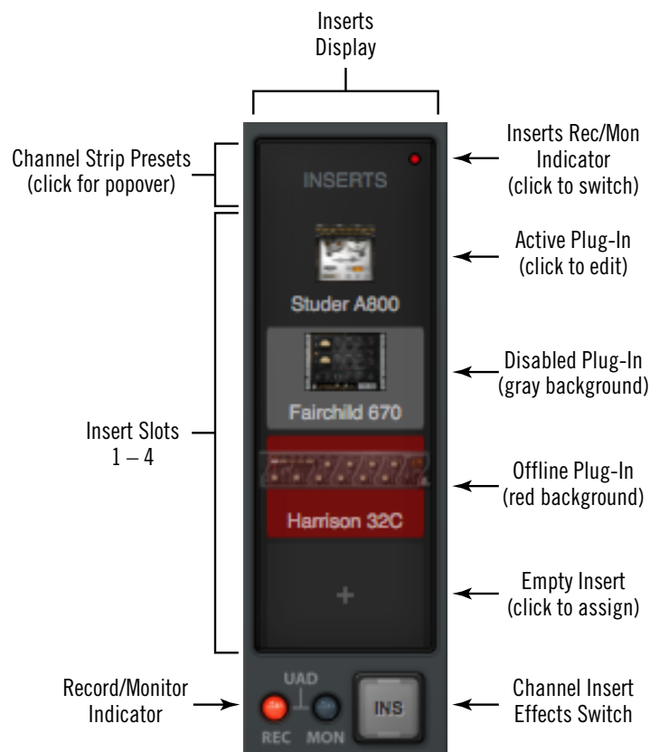
The Channel Inserts
