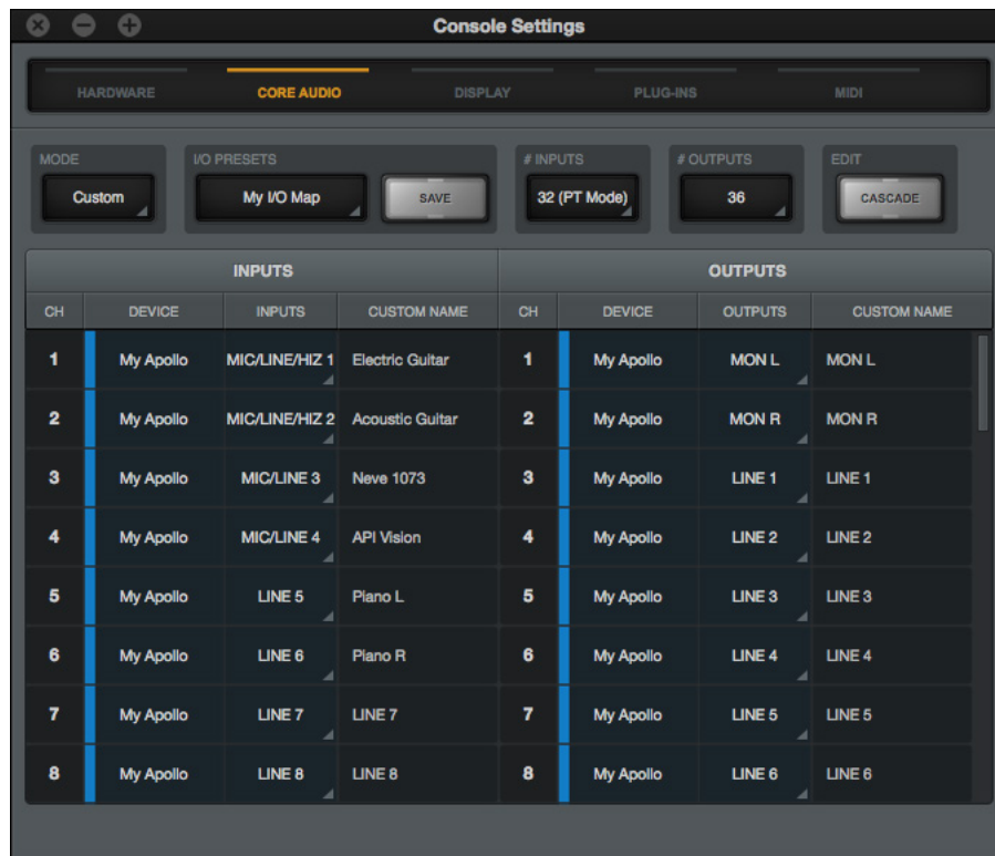
The Flex Driver feature is configured in the Core Audio settings panel
