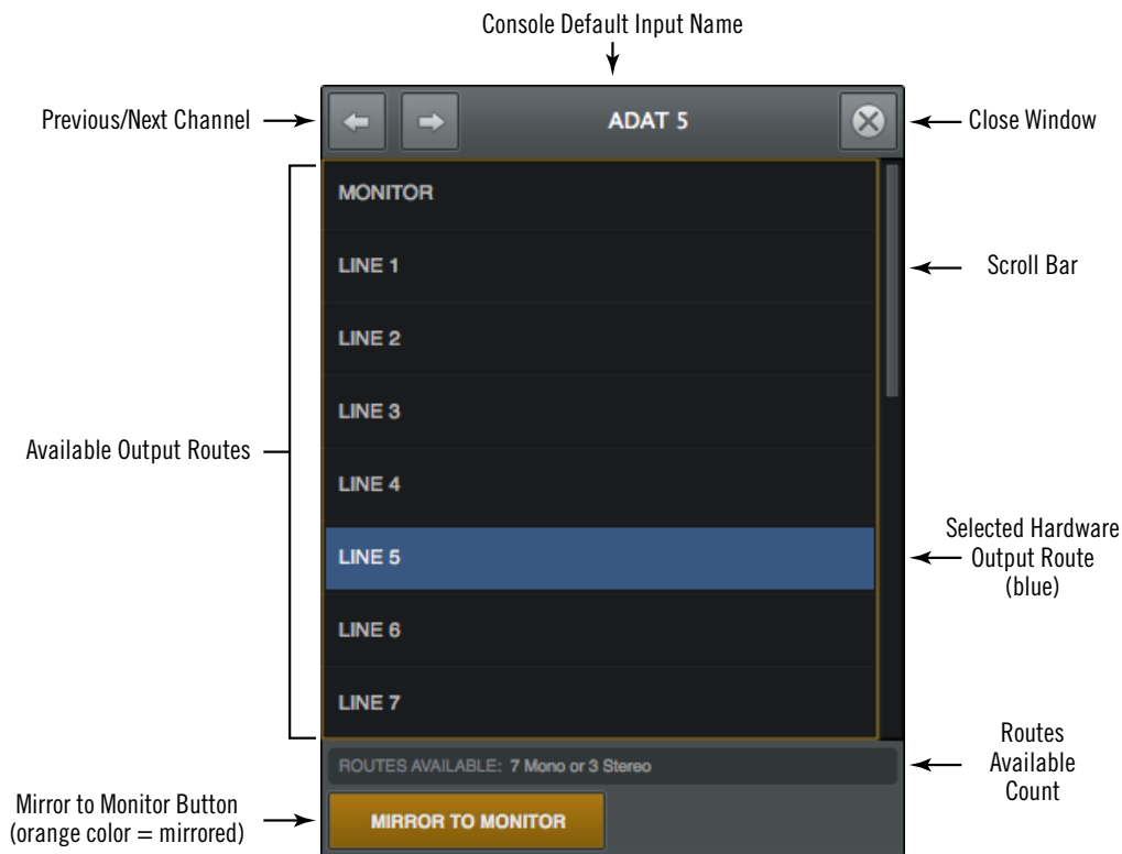
The Output Route popover
