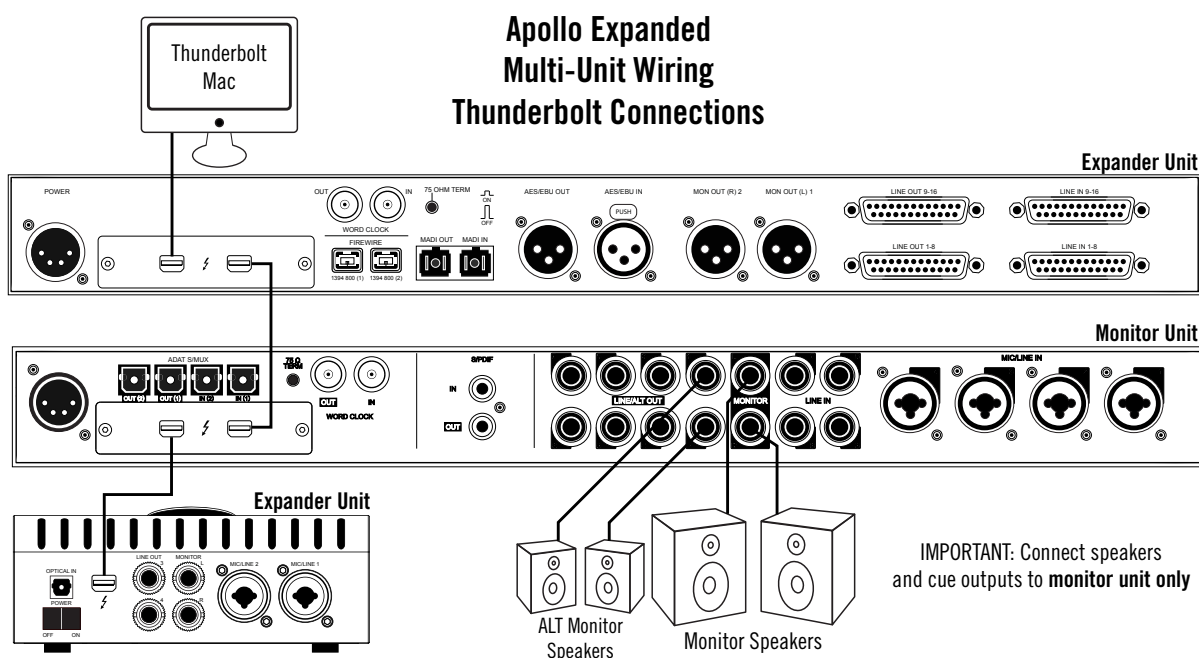
Device wiring example with Apollo 8, Apollo 16, and Apollo Twin
