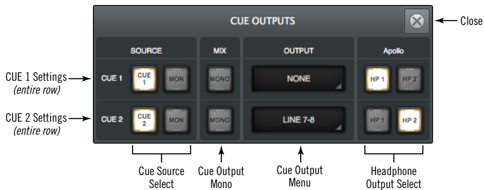
The Cue Outputs popover with Apollo, Apollo 8, Apollo 8p
