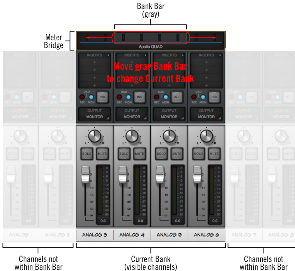
Conceptual illustration of the Current Bank. In this example, the Current Bank is analog channels 3 through 6. Moving the Bank Bar brings different channels into the Current Bank view.
