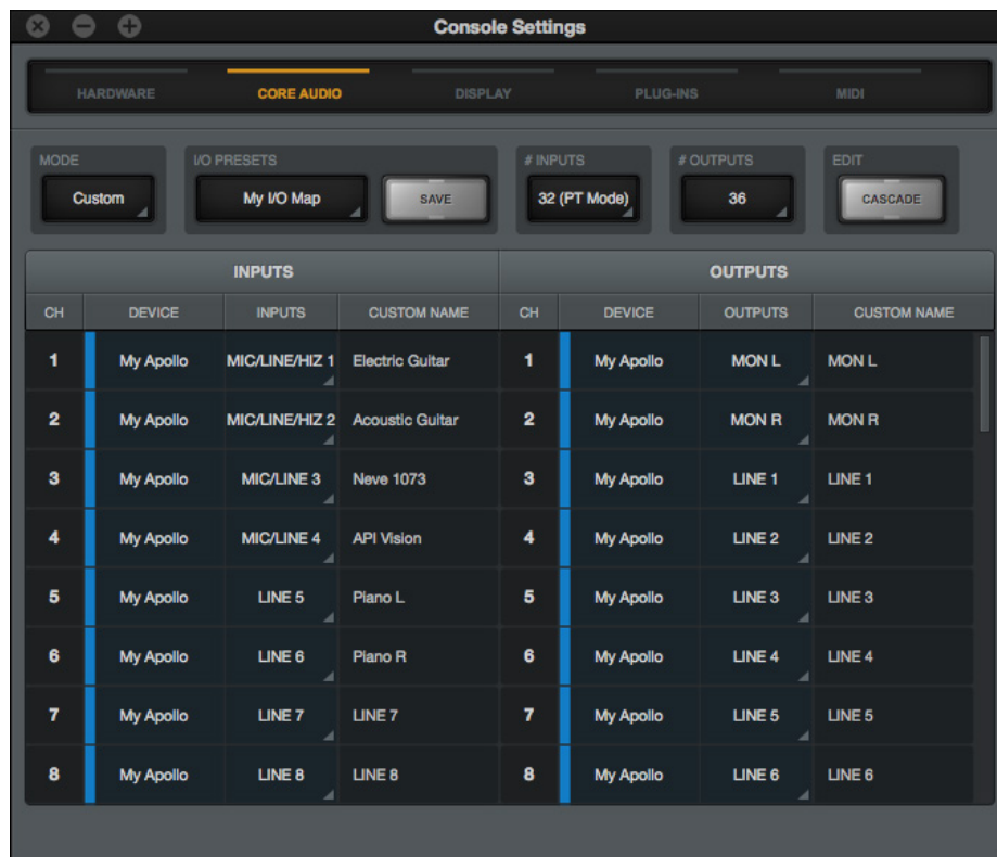
The Core Audio Panel
