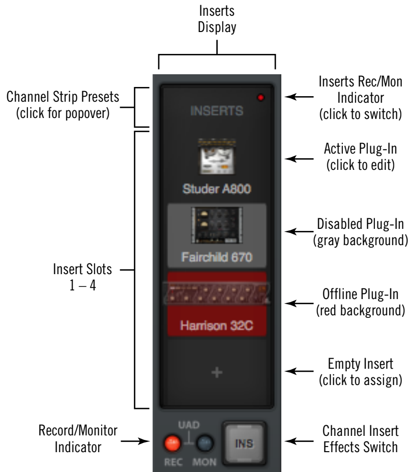
The Channel Inserts
