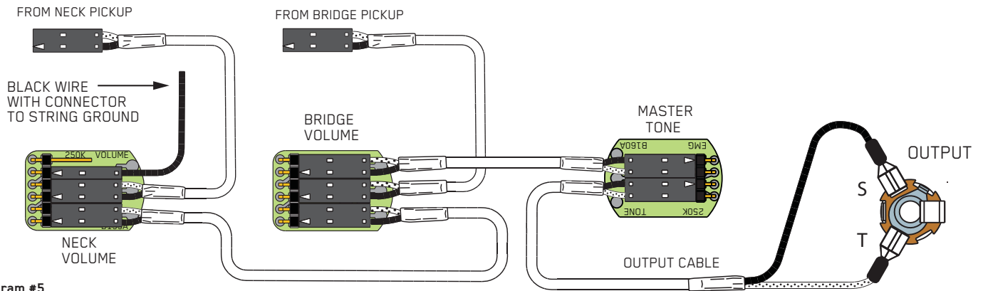
Diagram #5 2 Pickups Volume / Volume/ Tone
