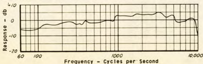
Fig. B. Typical Frequency Response, Series "556" Microphones
