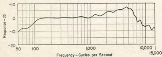
Response-Frequency Characteristic Model 55s Microphone. 27A02, 5-51.
