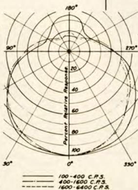
Horizontal Polar Response Series 556 Microphones
