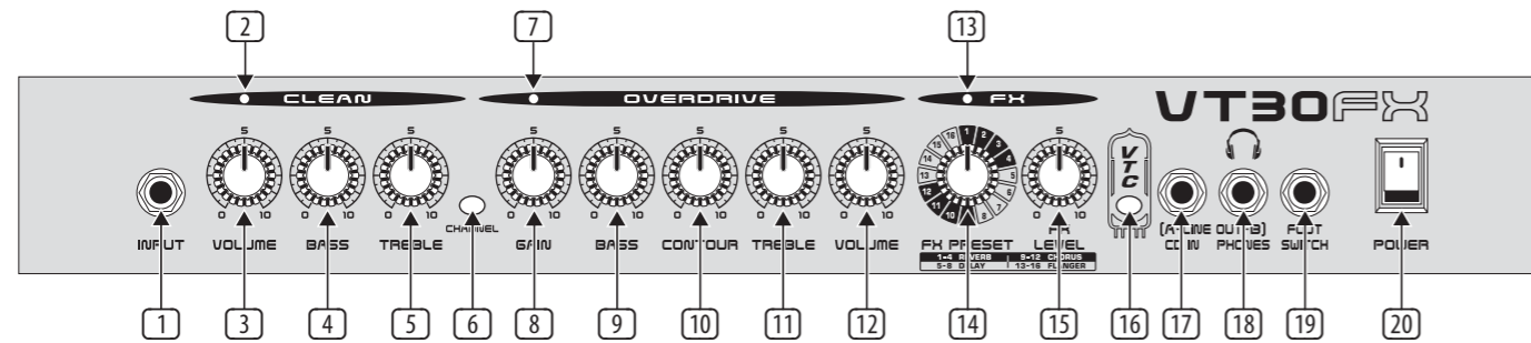
VIRTUBE control elements (front panel)
