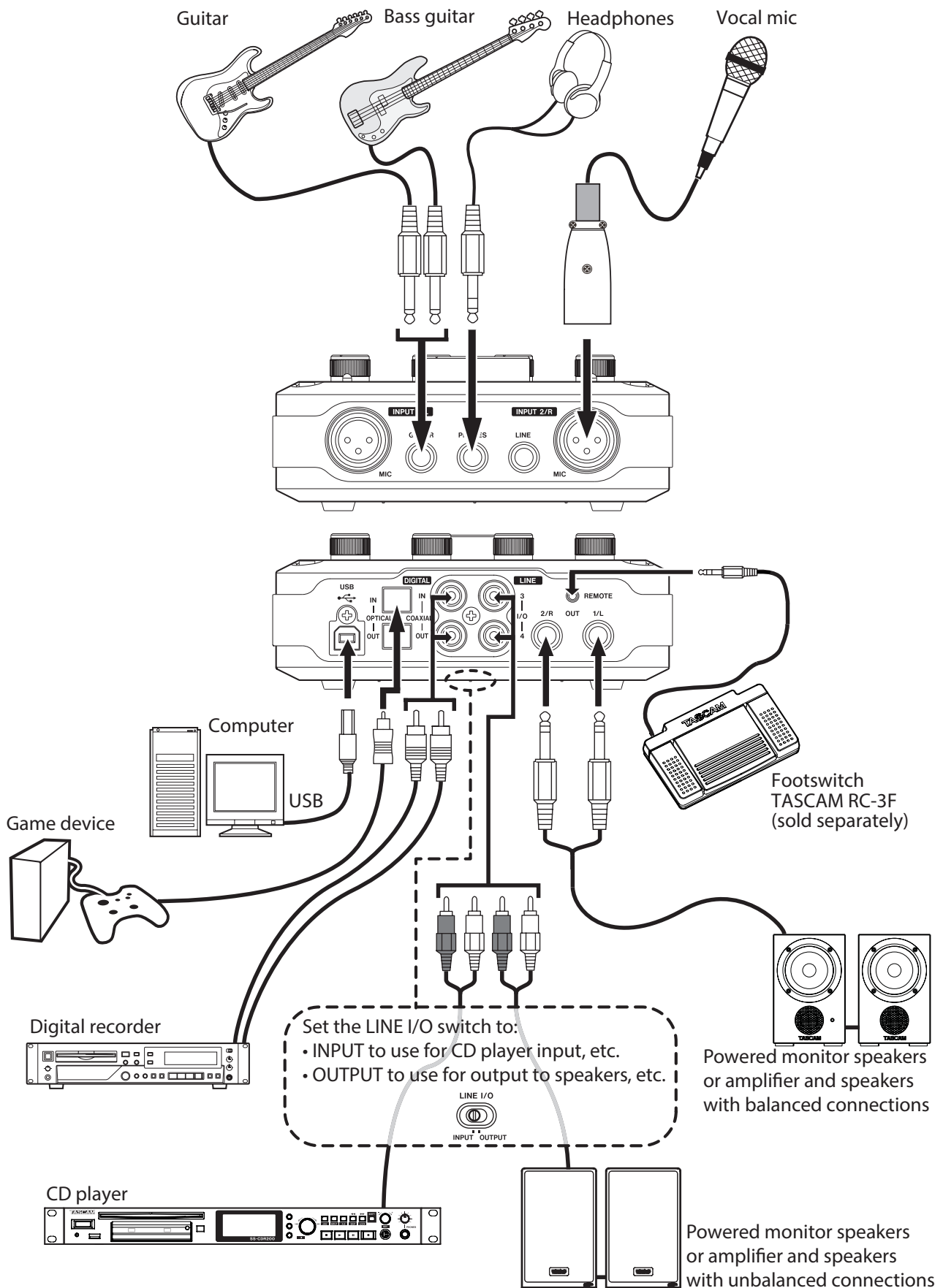
Example of using US-366 connections
