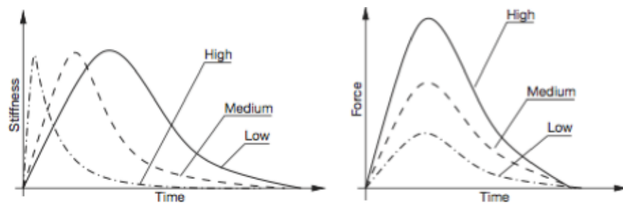
Figure 7: Effect of the Stiffness and Force knob on the output from the Hammer module.
