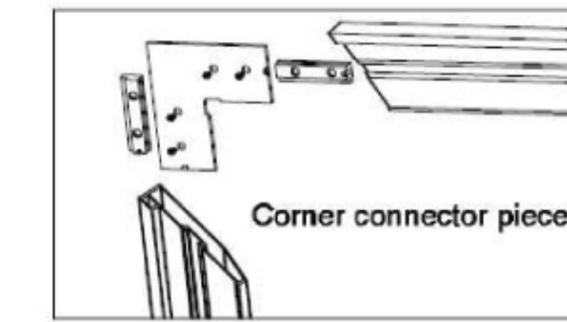
Corner connector pieces connect the outside of the frame
