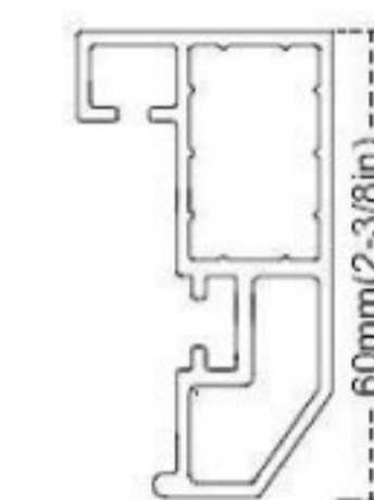
Signature Model corner connector piece side view
