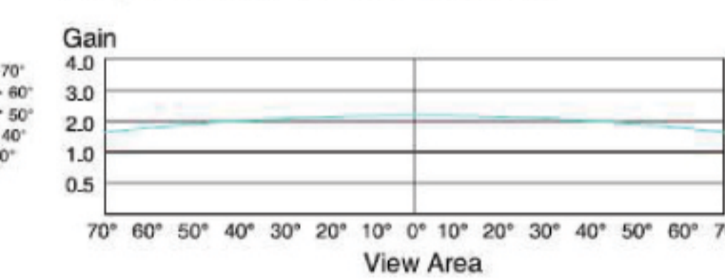
The gain of PS series Flexible Screen: 2.2
