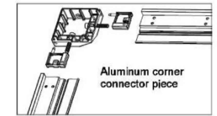
Aluminum corner connector pieces connect the outside of the frame
