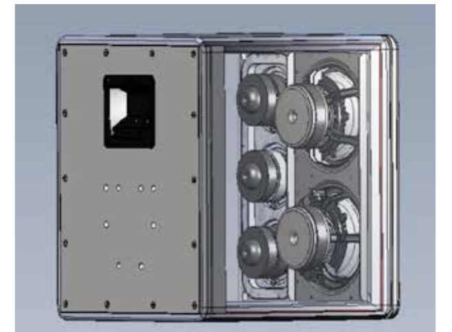
Dual 6.5" mid/woofers move air with a surface area greater than that of a single 9" woofer, but with far greater speed, precision, dynamic agility and power handling, because two separate cones and motor systems sharing the load run cooler and smoother.
