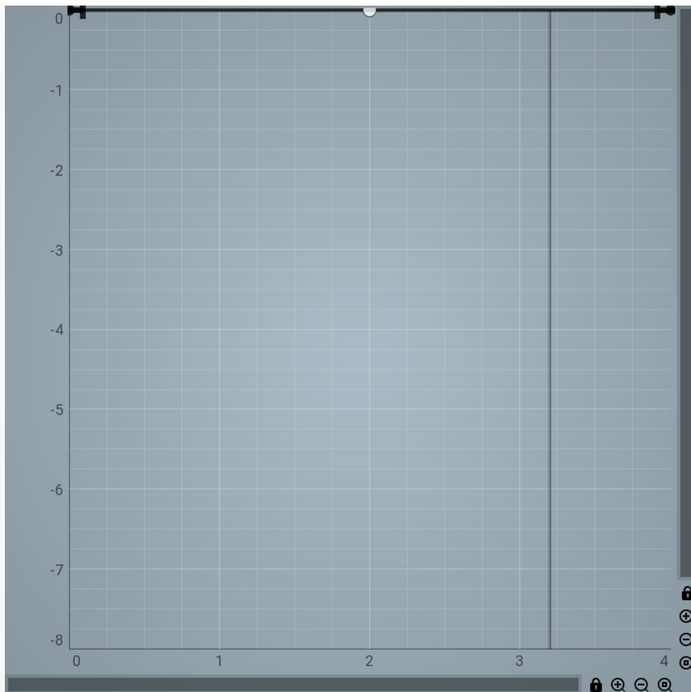
Graph editor
