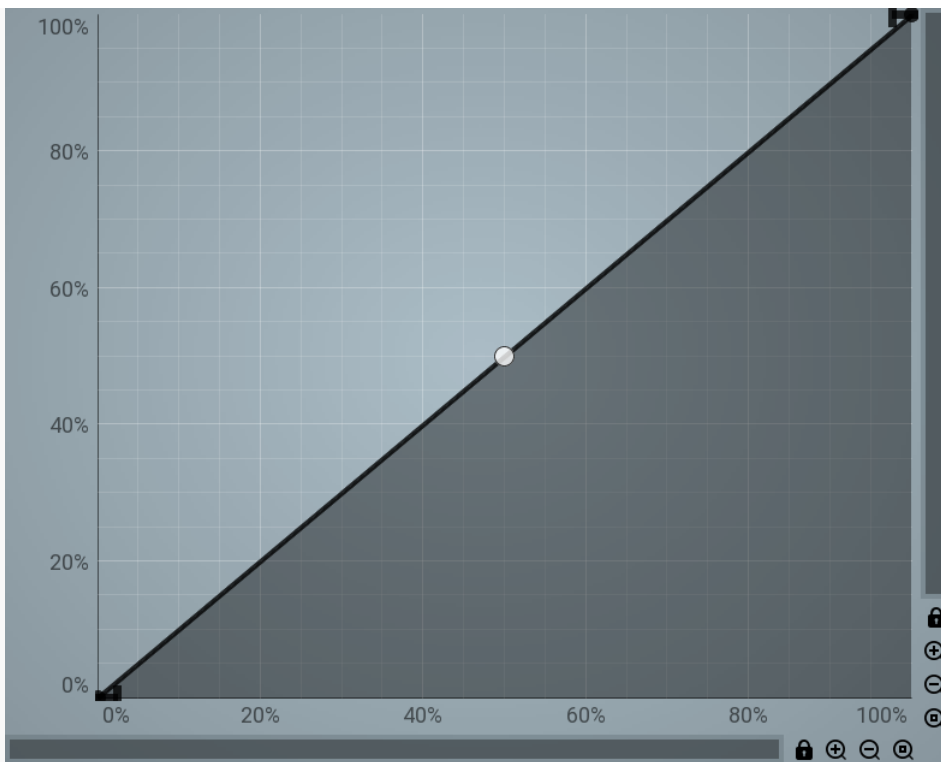
Graph editor
