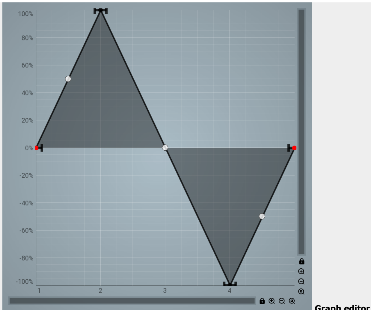
Graph editor
