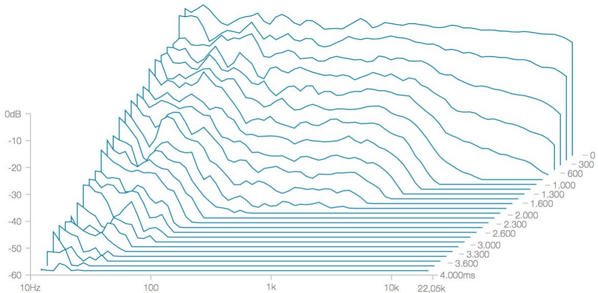
The effect of a crossover system with lows set to 200% and highs set to 50% of the decay time.
