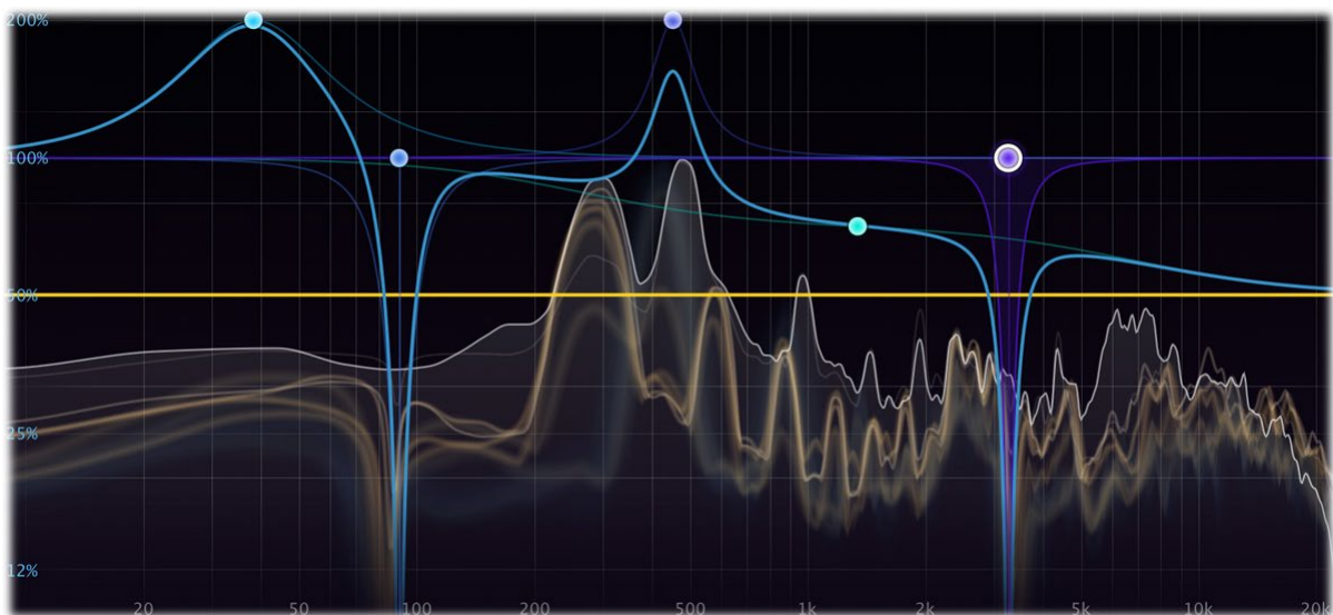
Using Pro-R's Decay Rate EQ, you can shape the decay time per frequency using Bell, Shelf and Notch curves...
