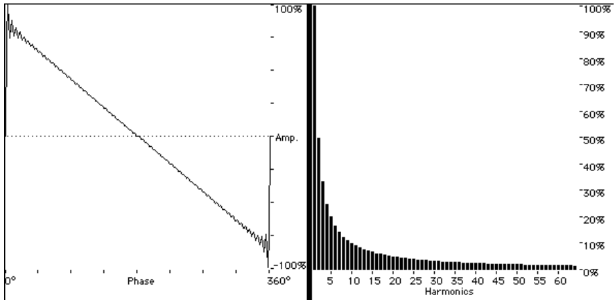
A saw (sawtooth) waveform, and the corresponding harmonic spectrum graphic. The saw wave has all the harmonics, in a special amplitude relationship.
