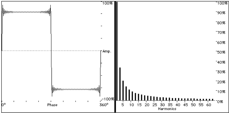
A square waveform, and the corresponding harmonic spectrum graphic. The square is a particular case of the pulse wave, where both positive and negative periods have the same value (50%). The harmonic graphic clearly shows the absence of even-numbered harmonics (only odd-numbered harmonics are present)
