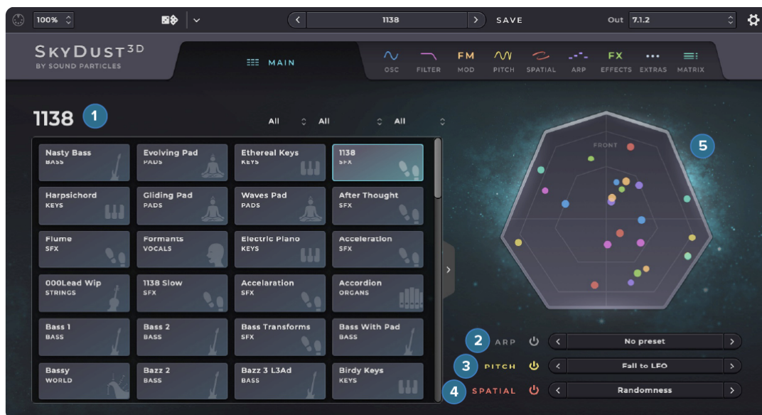
Figure 4. Main Page
