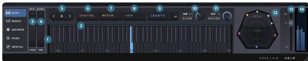
Figure 34. Keys Tab
