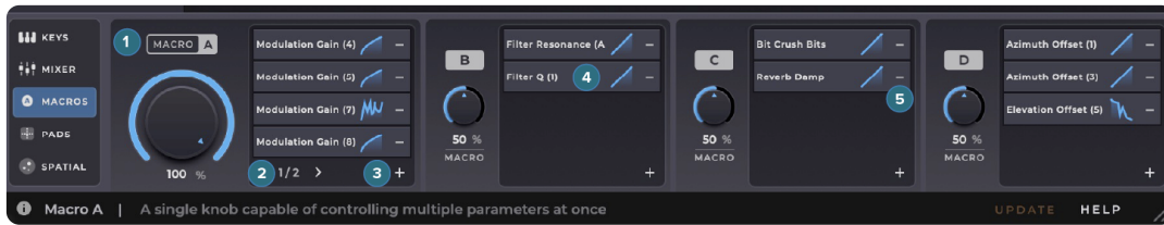
Figure 36. Macros Tab
