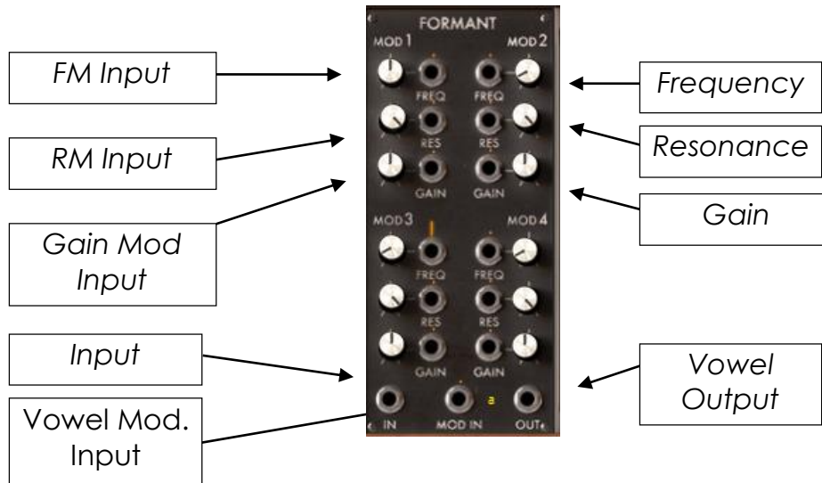
Formant filter
