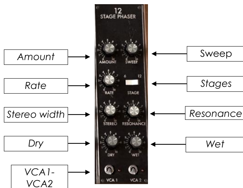
Phaser
