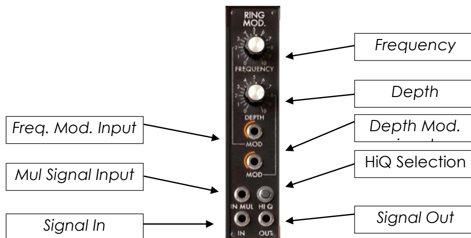
Ring modulator
