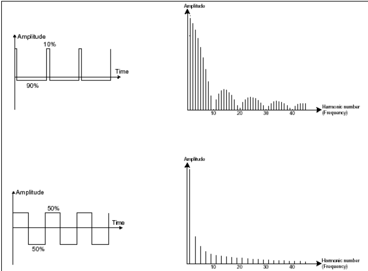
Square waveform
