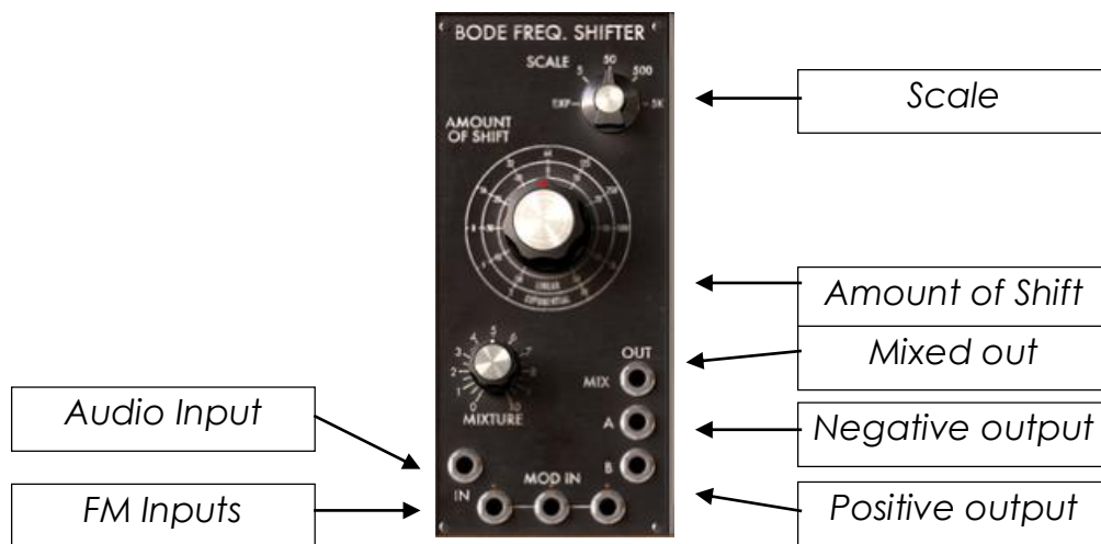
Bode frequency shifter
