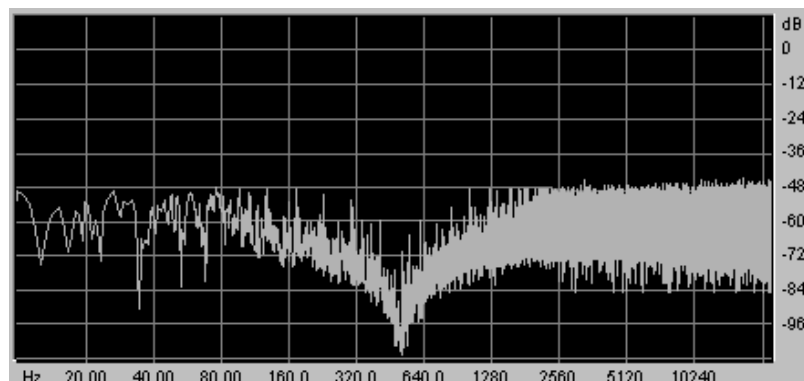
Band-reject filter
