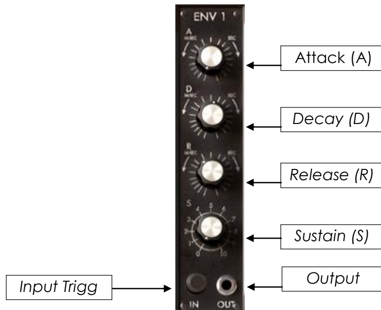
Envelope
