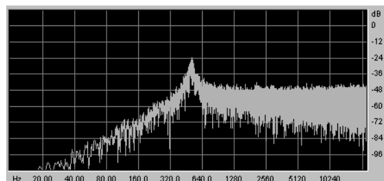
High-pass 12 dB/octave
