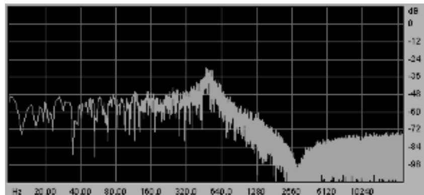
Low-shell filter
