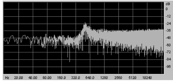
High-shelf 12 dB/octave
