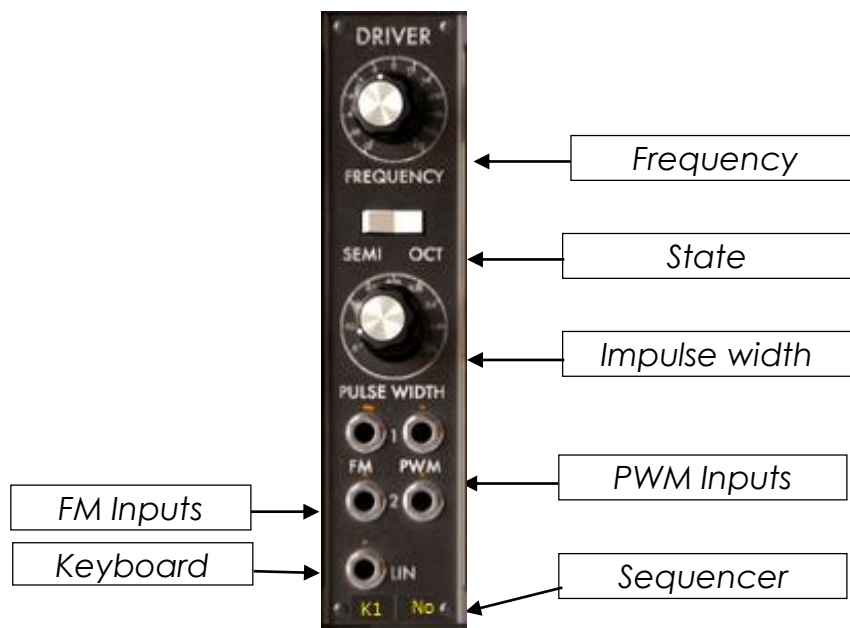
Oscillator 921A
