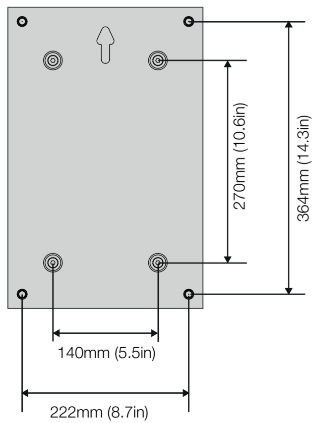
PLINTH BASE SCREW AND FOOT ALIGNMENT
