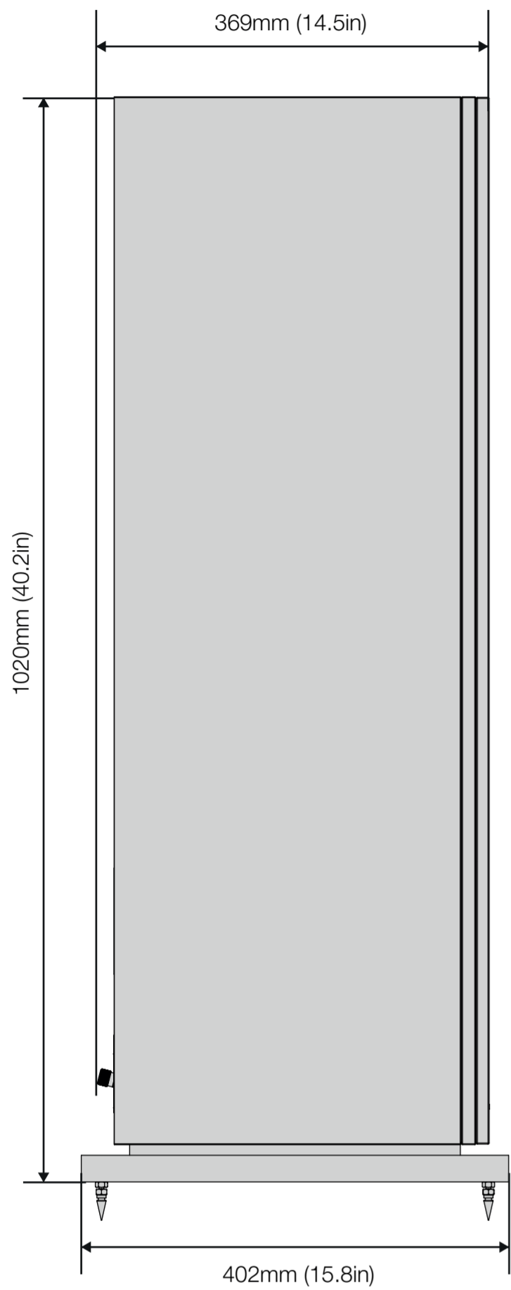
SIDE (WITH GRILLE)
